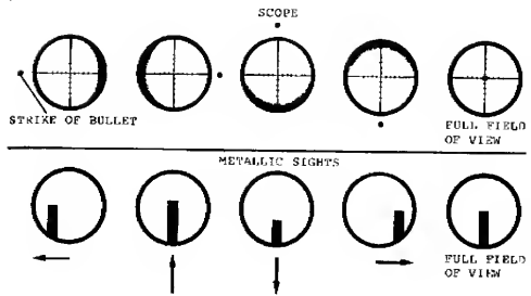
Figure 3-3. Sight alignment.
